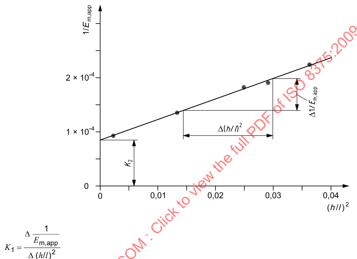
Figure 5 — Determination of shear modulus — variable span method
