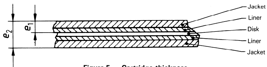
Figure 5 — Cartridge thickness
