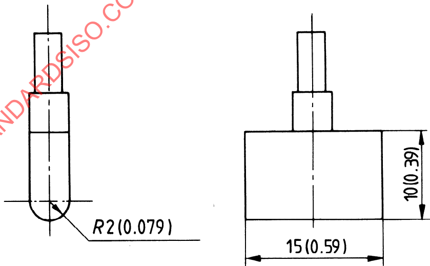
Figure 11 — Stylus
