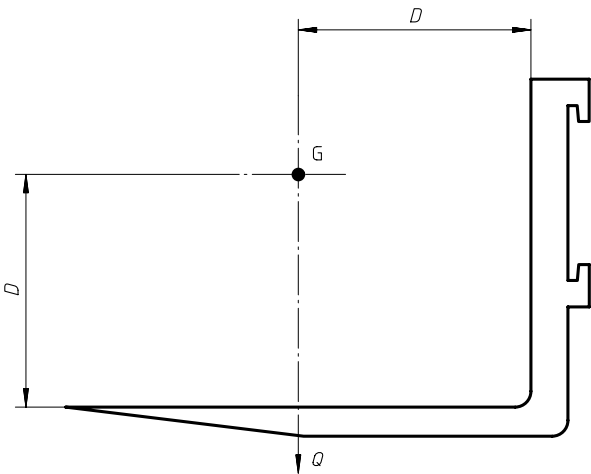
Figure 3 — Standard load distance centres
