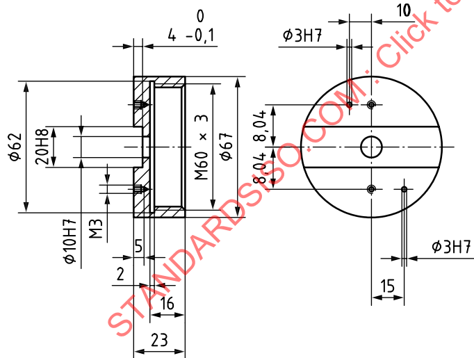
d) Orifice cap
