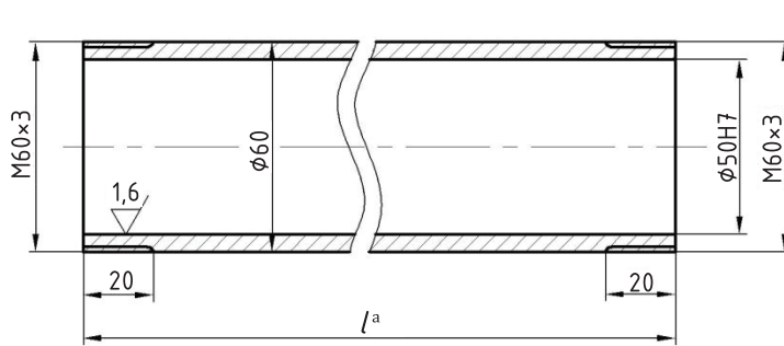
a) Cylinder
