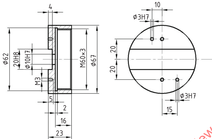
d) Orifice
