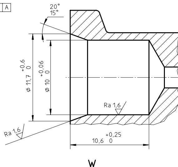
b) Socket on engine or gearbox flanges for use with accessory flanges having a transfer tube
