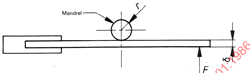
a) Schematic fixture for semi-guided bend test—one end held, force applied near free end
