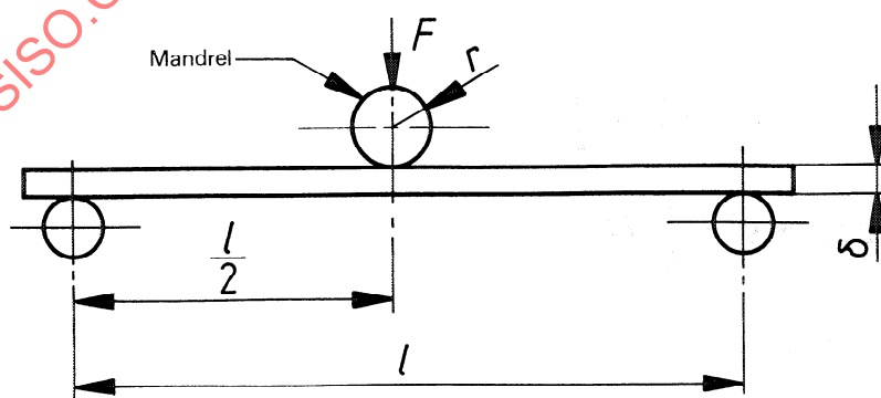
c) Schematic fixture for semi-guided bend test—ends supported
