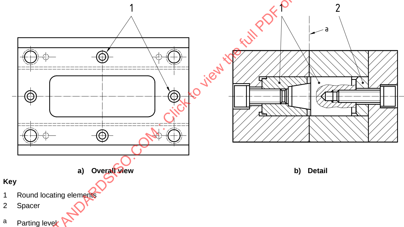
Figure 1 — Example of mounting of round locating elements
