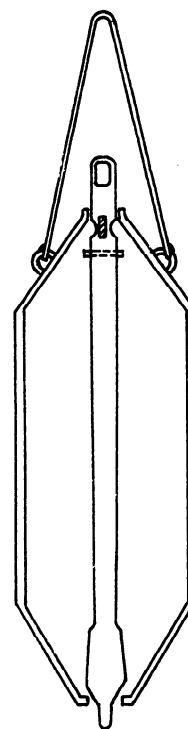
Figure 5 — Bottom or zone sampler (sectional view)
