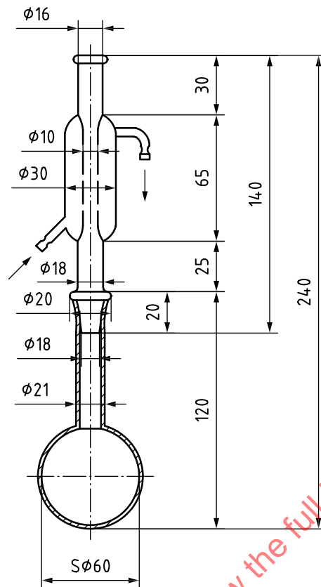
Figure 5 — Apparatus for corrosion
