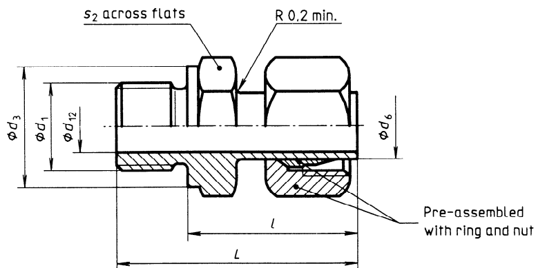
Figure 19 — Swivel adaptors (SW) for ports with elastomeric sealing
