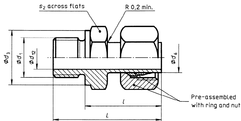
Figure 20 — Swivel adaptors (SW) for ports with metal-to-metal sealing
