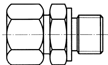
ISO 8434-1 - SDS - S20 × G 3/4 A
