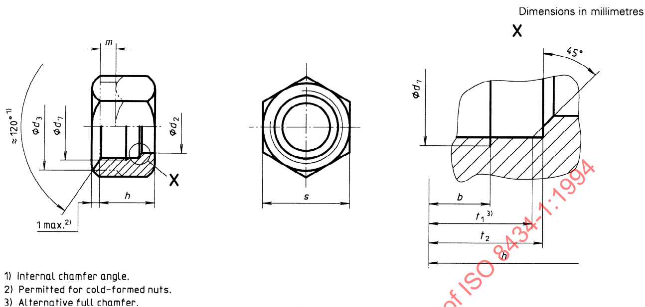
Figure 8 — Tube nuts (N)
