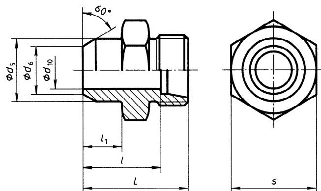
Figure 17 — Weld-on fittings (WDS)
