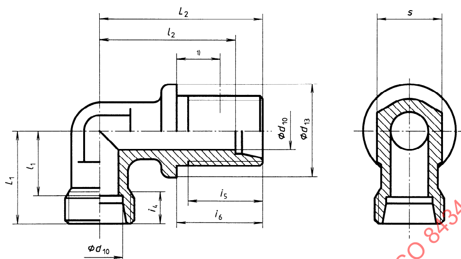
Figure 15 — Bulkhead elbows (BHE)
