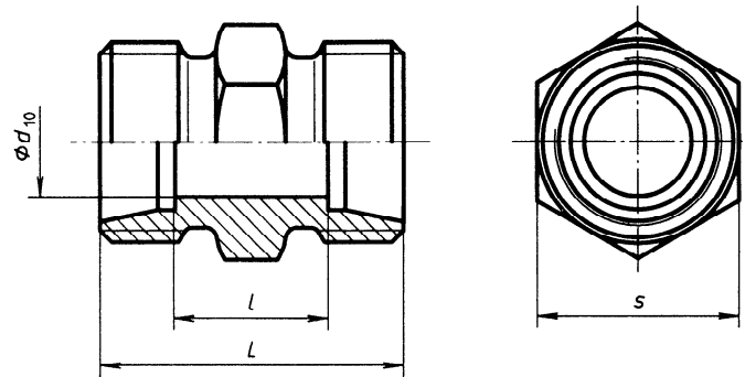
Figure 9 — Straight union fitting (S)
