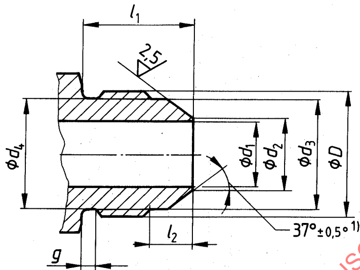
Figure 2 — 37° flare fitting
