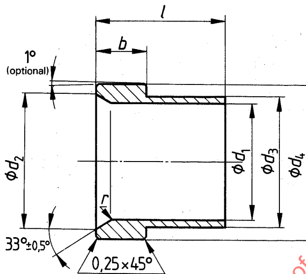
Figure 4 — 37° sleeve
