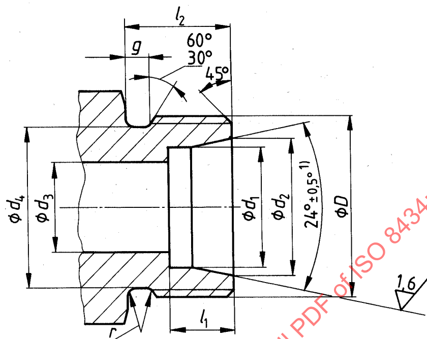
• Figure 1 — 24° flareless (bite) fitting
