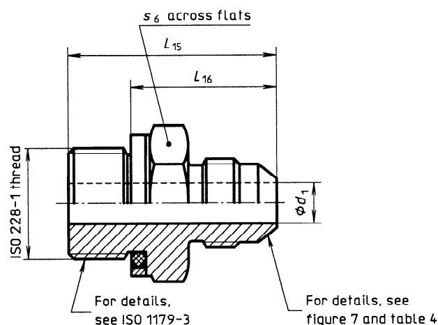
Figure 13 — Stud fitting (SDS) with ISO 1179-3 non-adjustable stud ends
