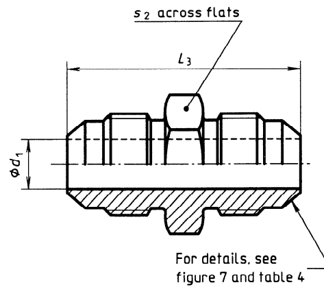
Figure 11 — Straight union fitting (S)
