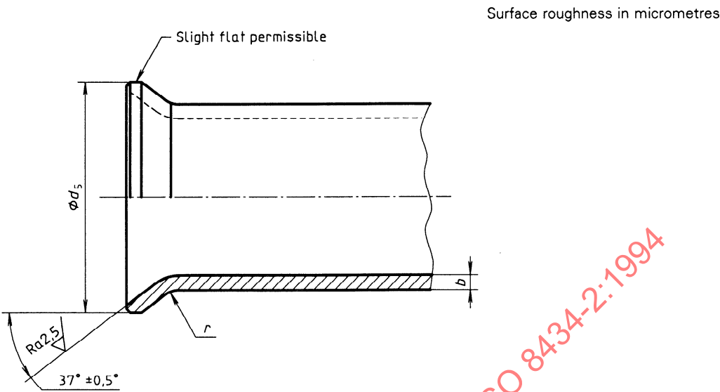
Figure 8 — 37° flare for tubes
