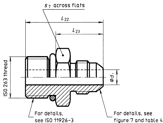
Figure 16 — Stud fitting (SDS) with ISO 11926-3 non-adjustable stud ends
