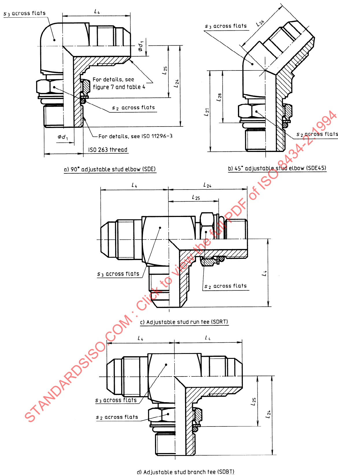
Figure 17 — Stud fittings with ISO 11926-3 adjustable stud ends
