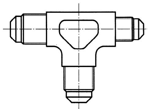
ISO 8434-2 - RERT - 20 × 12 × 20
