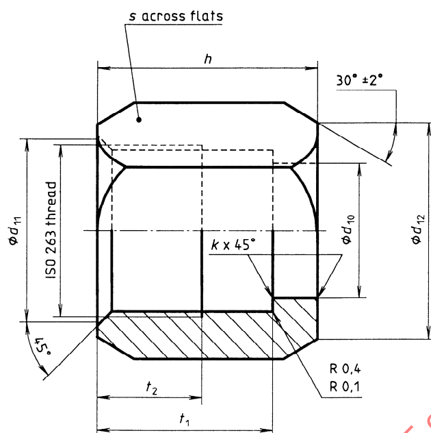
Figure 10 — Tube nut (N)
