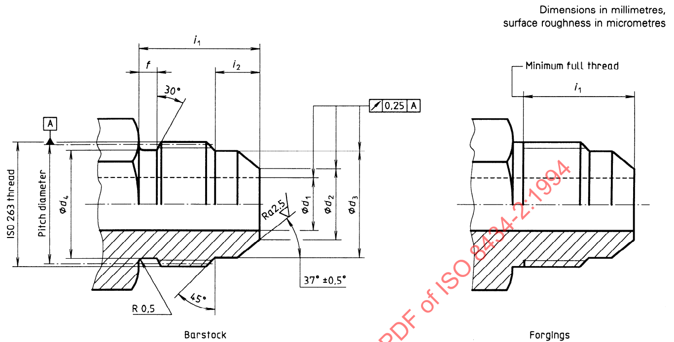
Figure 7 — 37° flared fitting connection
