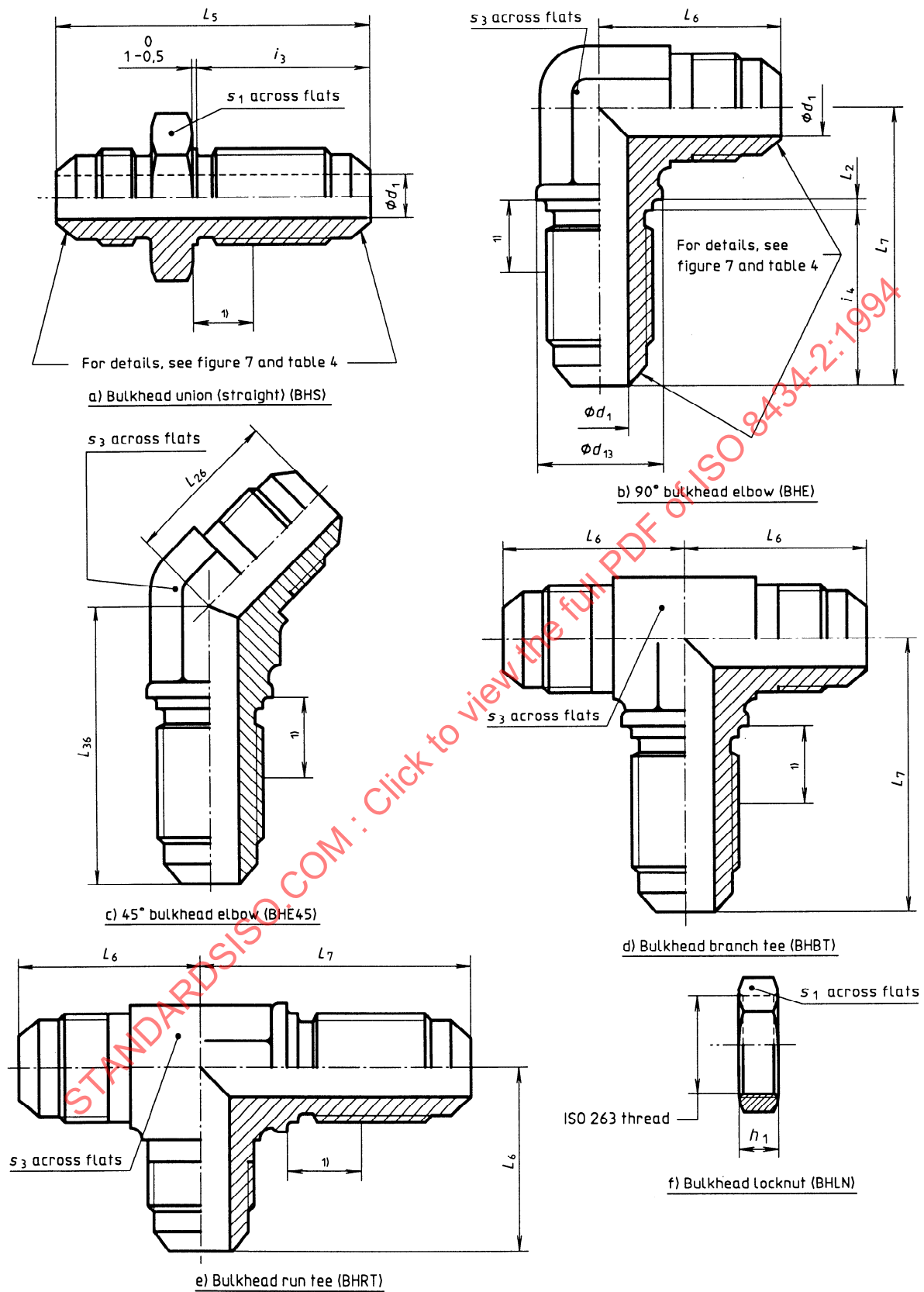
Figure 18 — 37° flared bulkhead union fittings and locknuts
