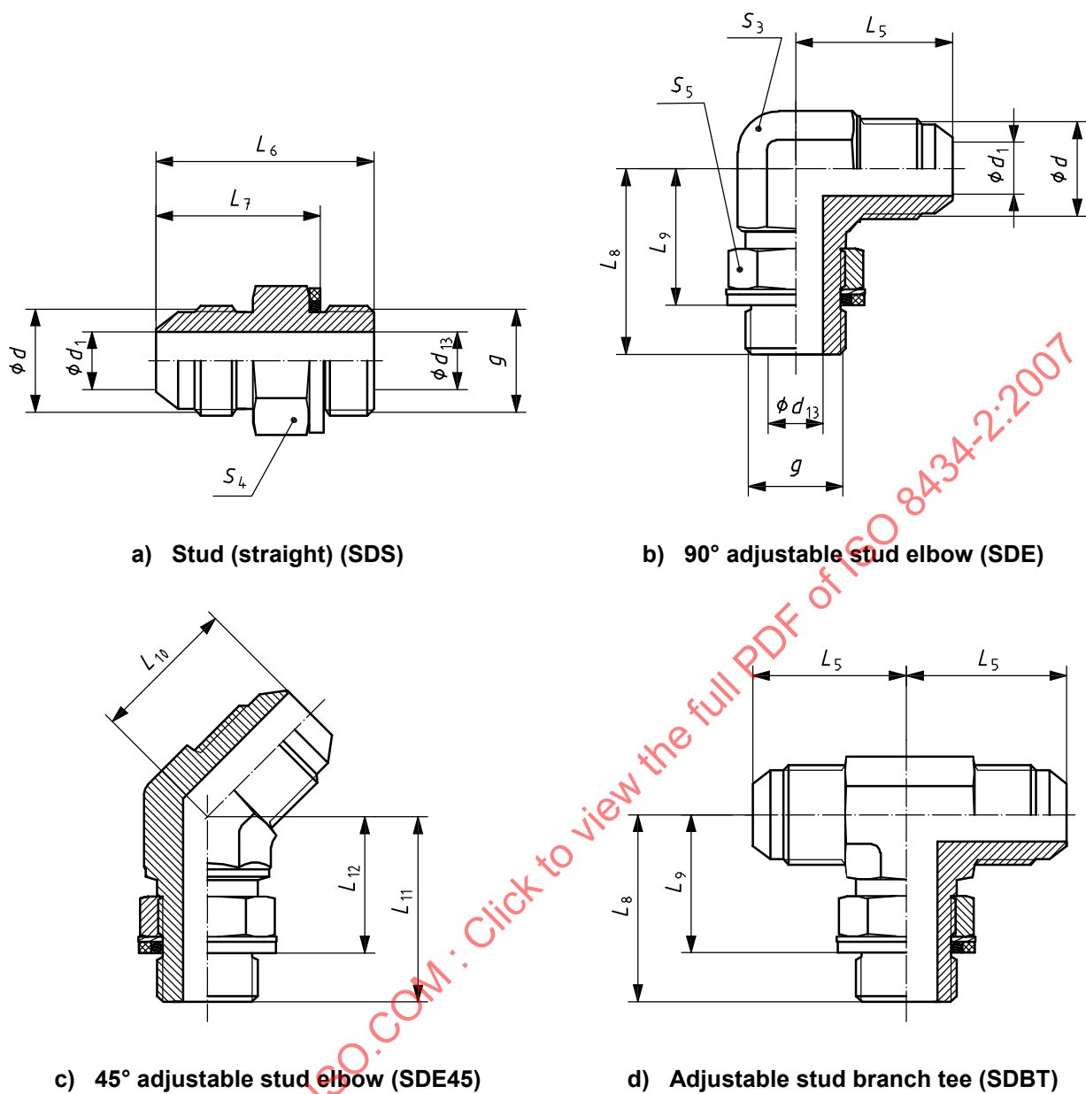
Figure 10 — Stud connectors with ISO 1179-3 stud ends
