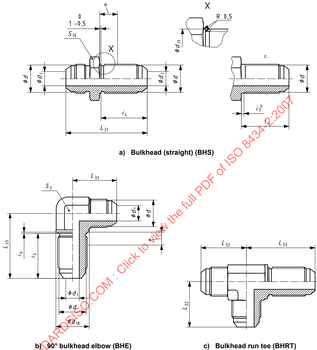
Figure 15 — Bulkhead connectors and corresponding bulkhead locknuts
