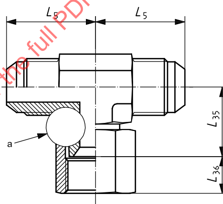
c) Swivel branch tee (SWBT)
