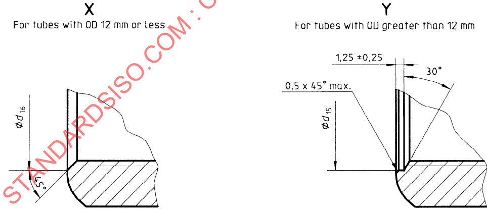
Figure 4 — Standard tube nut (NA) and high-strength tube nut (NB)
