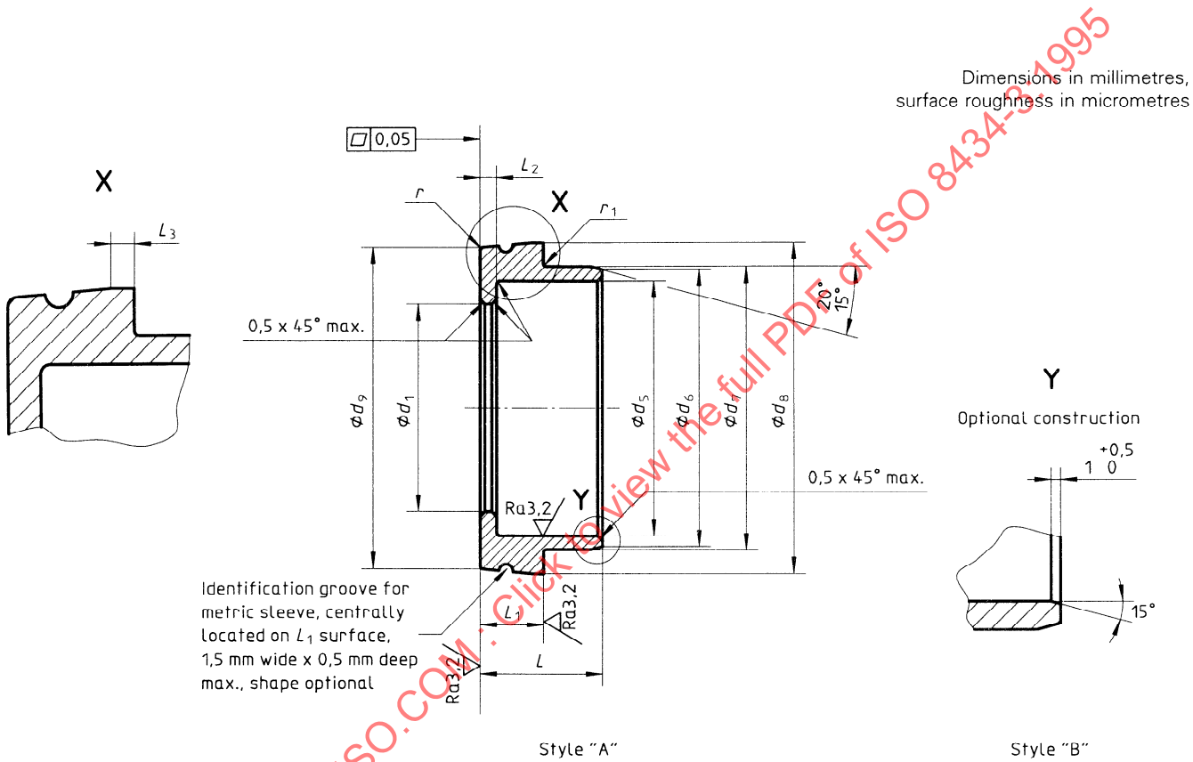
Figure 3 — Braze sleeve [BRSL-A (standard) and BRSL-B (option)]
