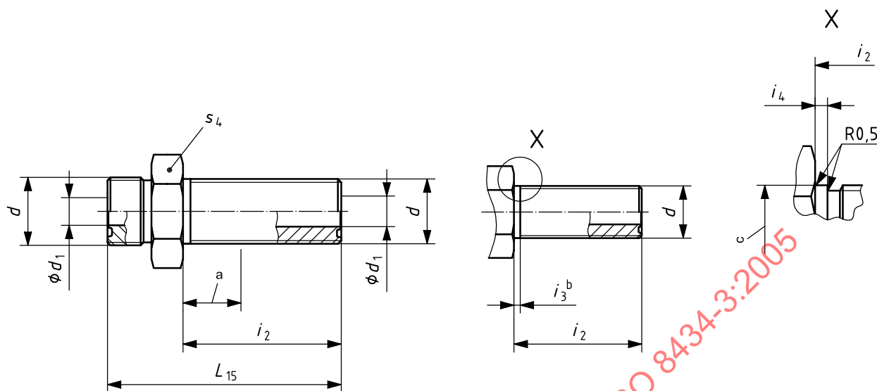
a) Bulkhead (straight) (BHS)
