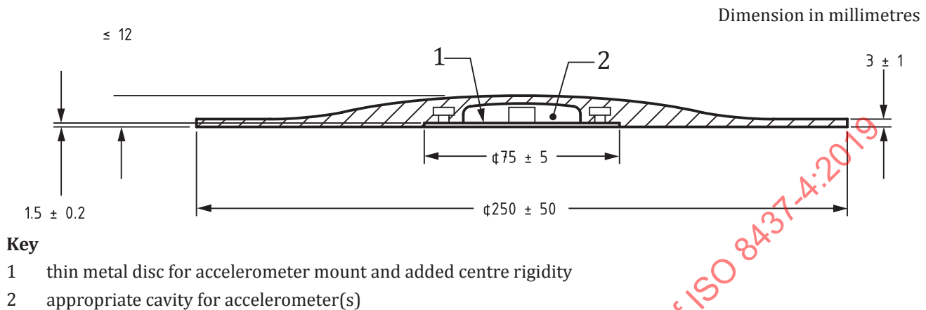
Figure B.1 — Design of a semi-rigid mounting disc
