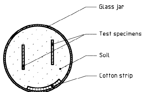
Figure 1 — Arrangement of test specimens in the soil in soil-burial tests (cross-section)
