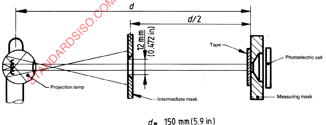
Figure 10 — Measuring device
