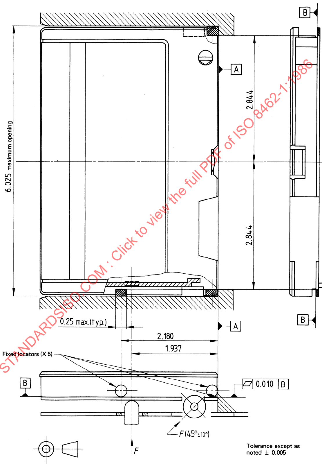
Figure 4b) — Cartridge locating planes
