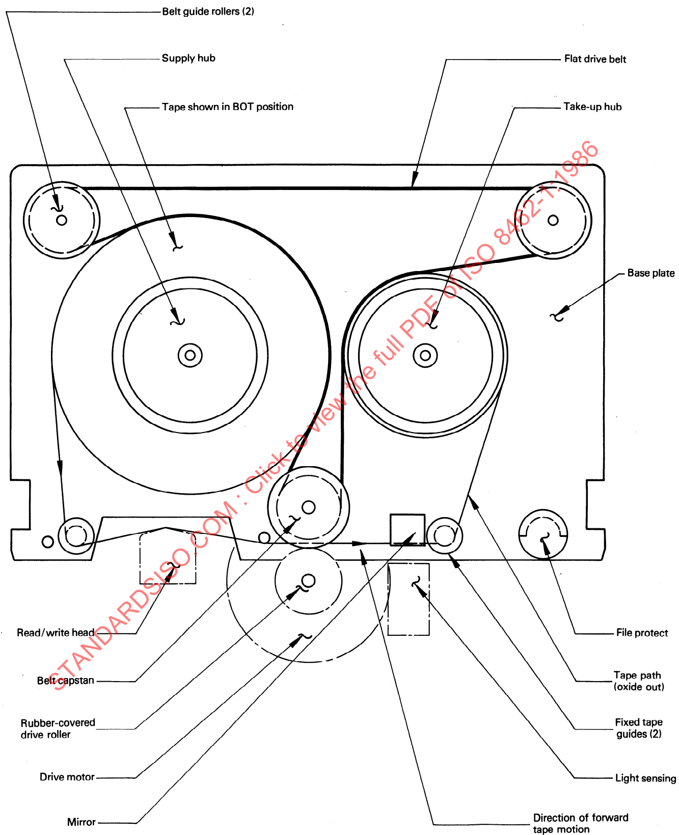
Figure 2 — Cartridge diagram
