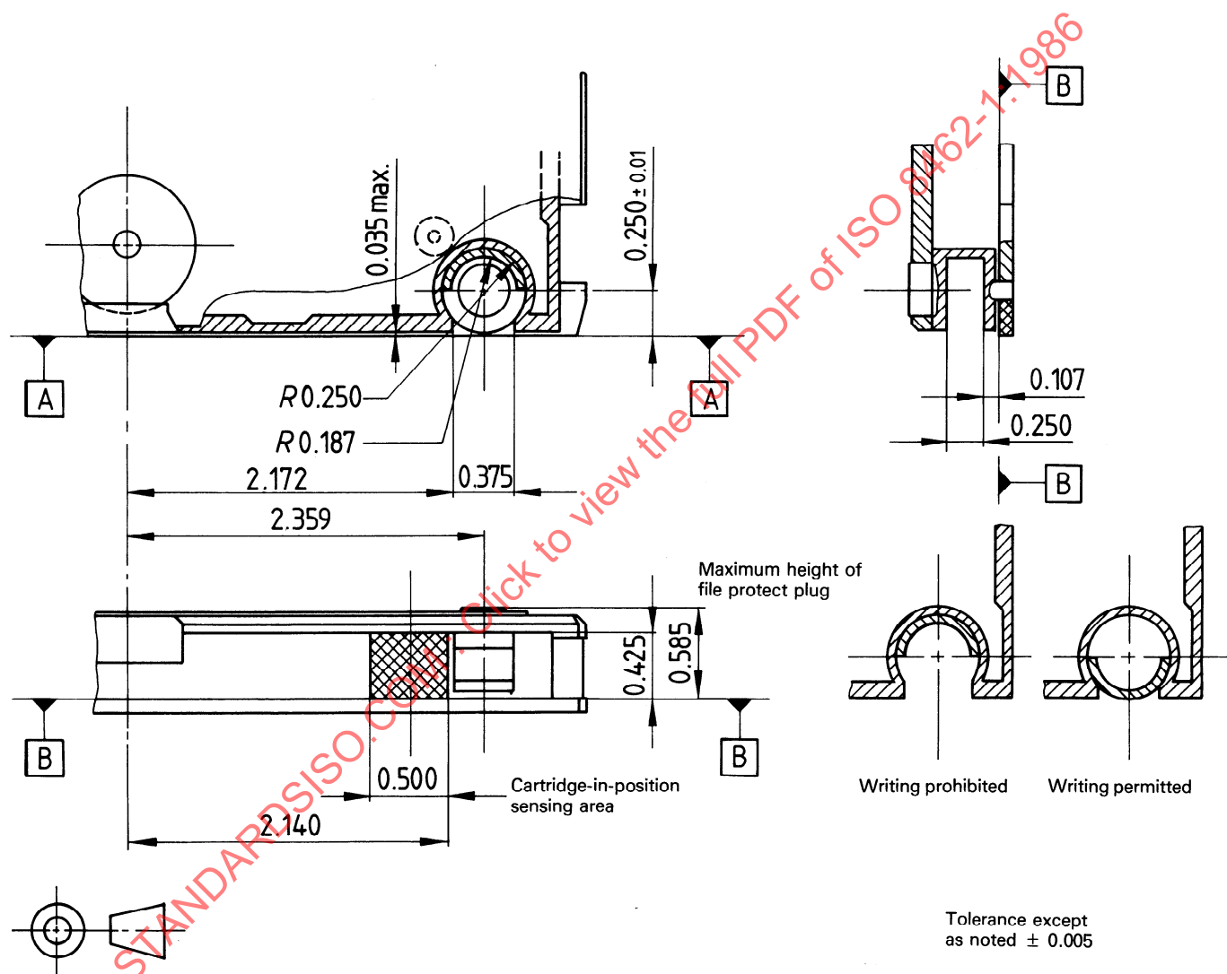
Figure 6b) — File protect and cartridge-in-position sensing
