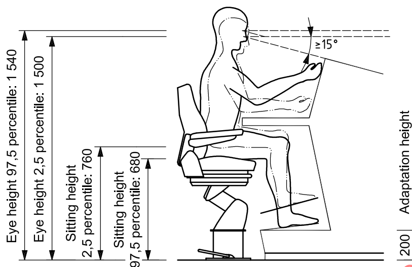
Figure 12 — Typical dimensions for seated position
