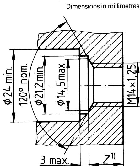
Figure 2 — Housing of spark-plug in cylinder head
