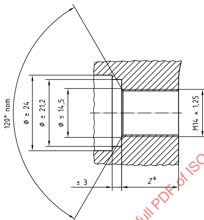
Figure 2 — Cylinder head housing
