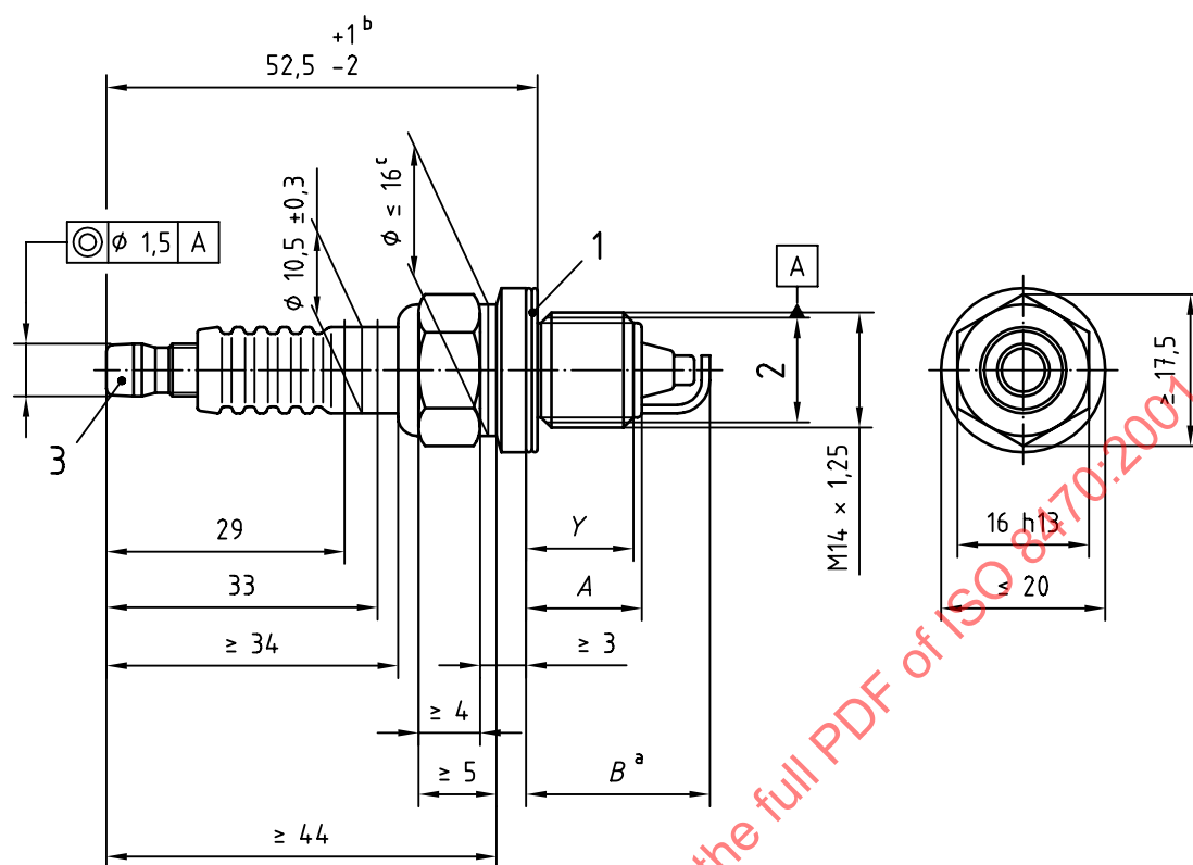
a) With solid post terminal
