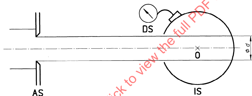
a) Measuring incident radiant flux
