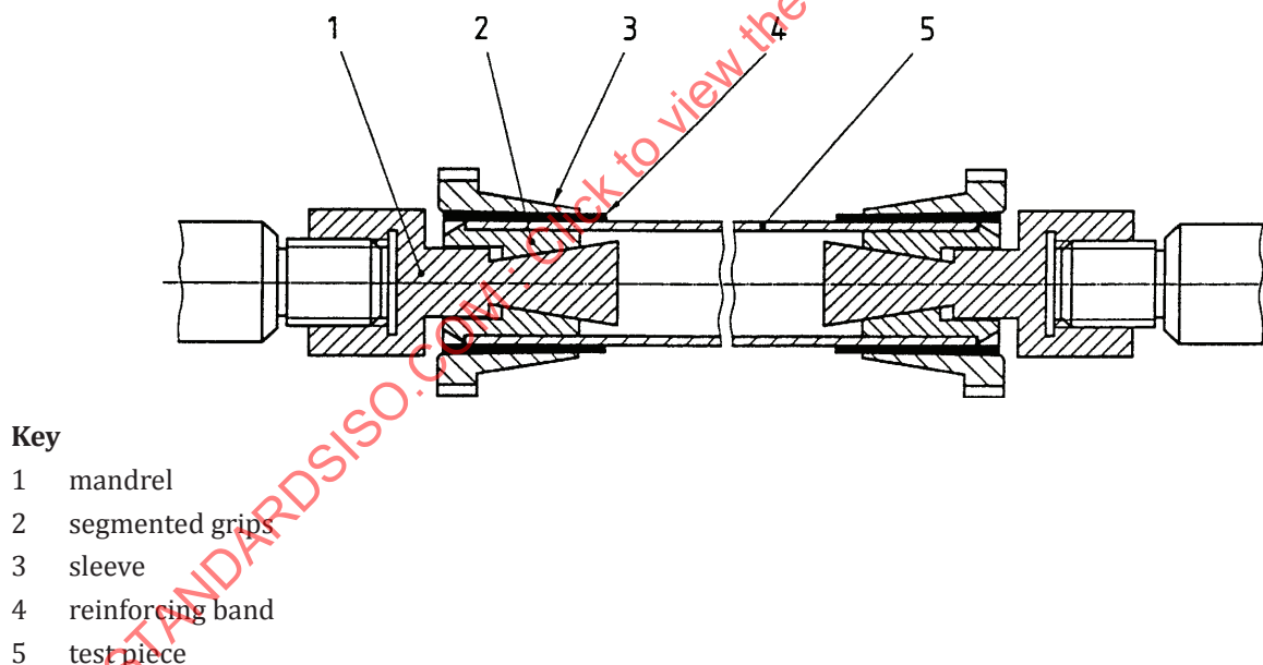
Figure 1 — Typical grips for a pipe section test piece (method B)
