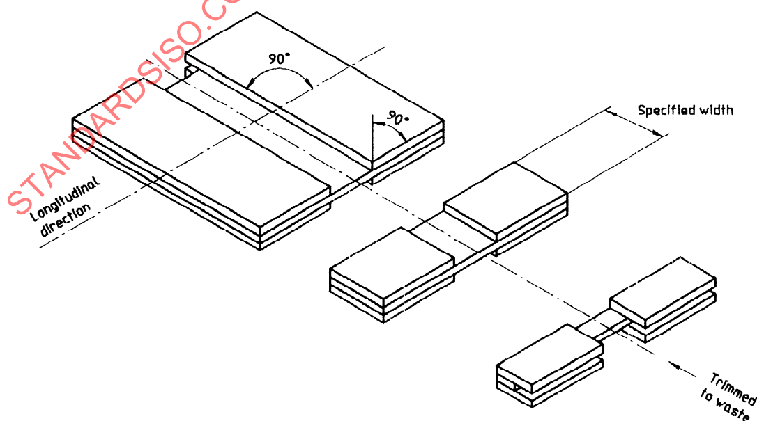
Figure 4 — Arrangement of specimen and end pieces for method A
