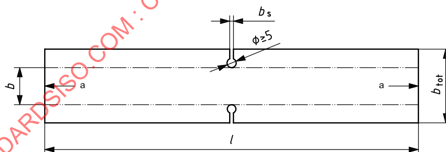
b) Case 2 - applies when helically wound layers are present in the test piece
