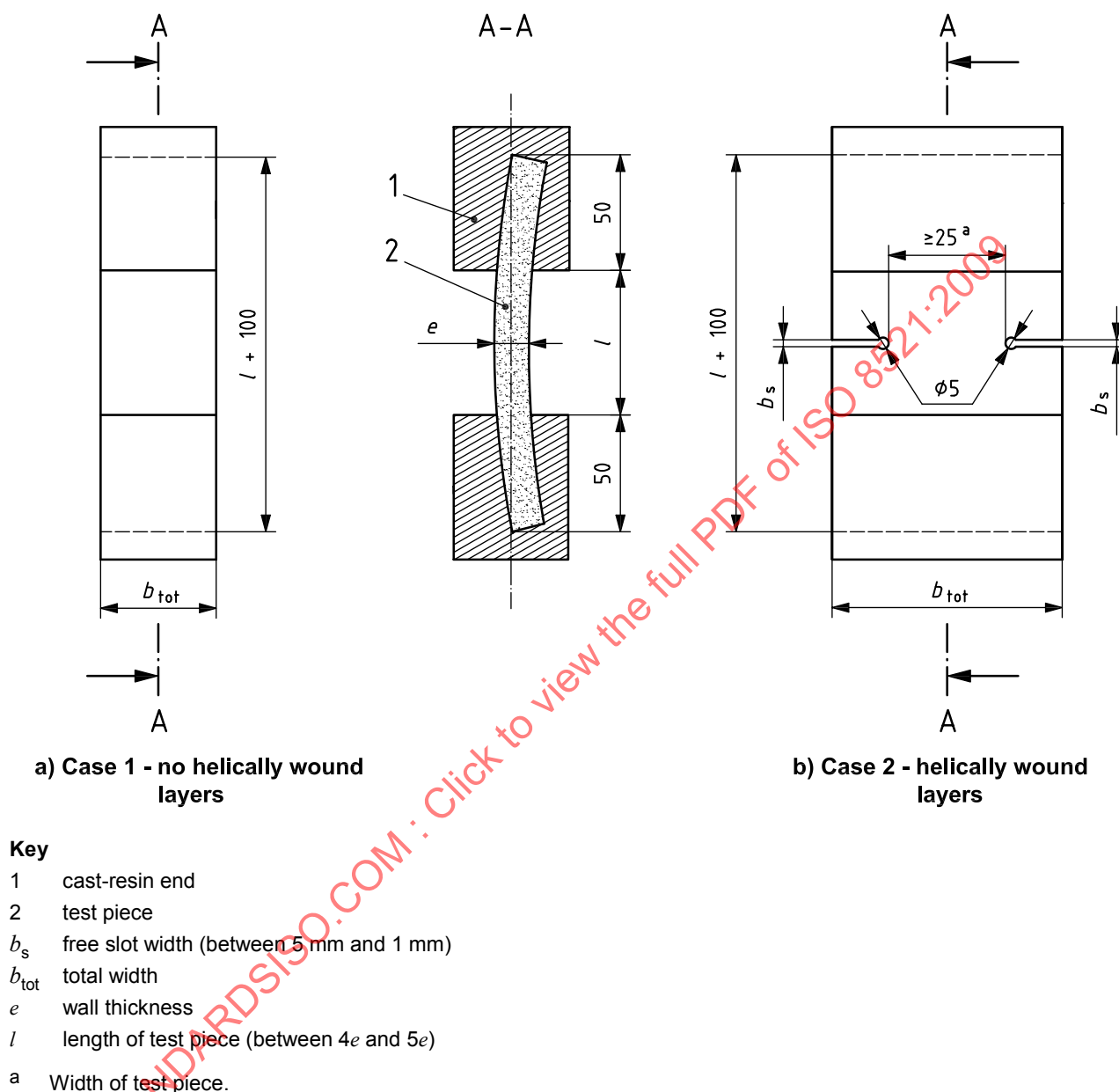
Figure 5 — Test piece for strip test (method C)
