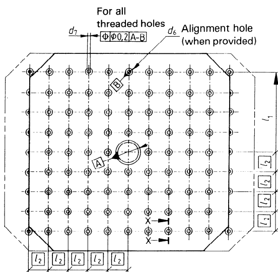
a) top surface, type 1 — with threaded fixing holes
