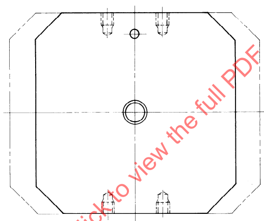
Figure 5 — Fixing holes for latch mechanism (the pallet illustrated is of type 4 with plain top surface)
