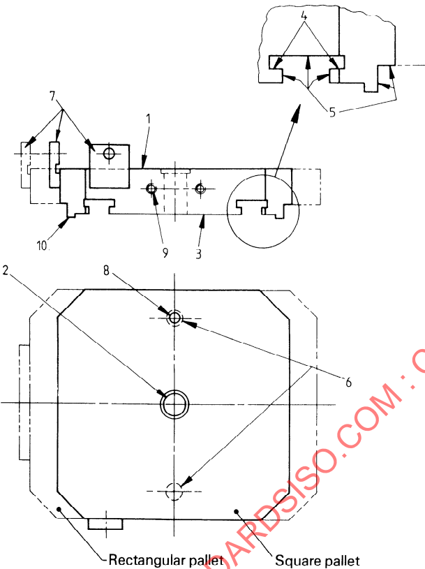
Figure 1 — Workholding pallet
