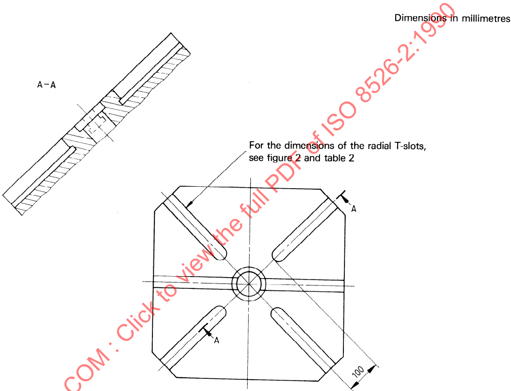
Figure A.1 — Top surface, type 5 — with radial T-slots
