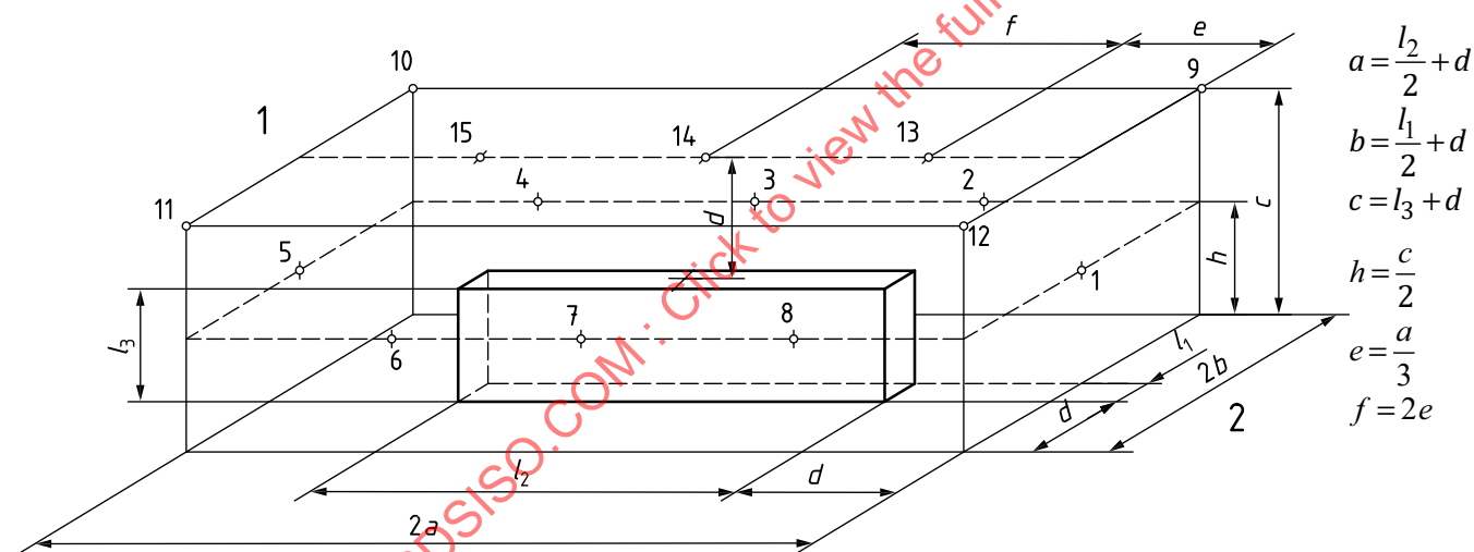
Figure A.3 — Measuring point arrangement (12 measuring points) and measuring plane for generating sets with the reference box measurements: 2 \text{ m} < l_2 \leq 4 \text{ m} and l_3 \leq 2,5 \text{ m}
