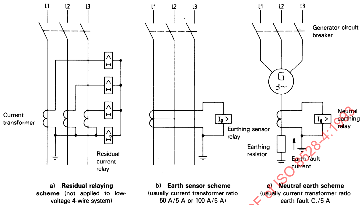
Figure 3 — Earth-fault protection detecting zero-sequence current
