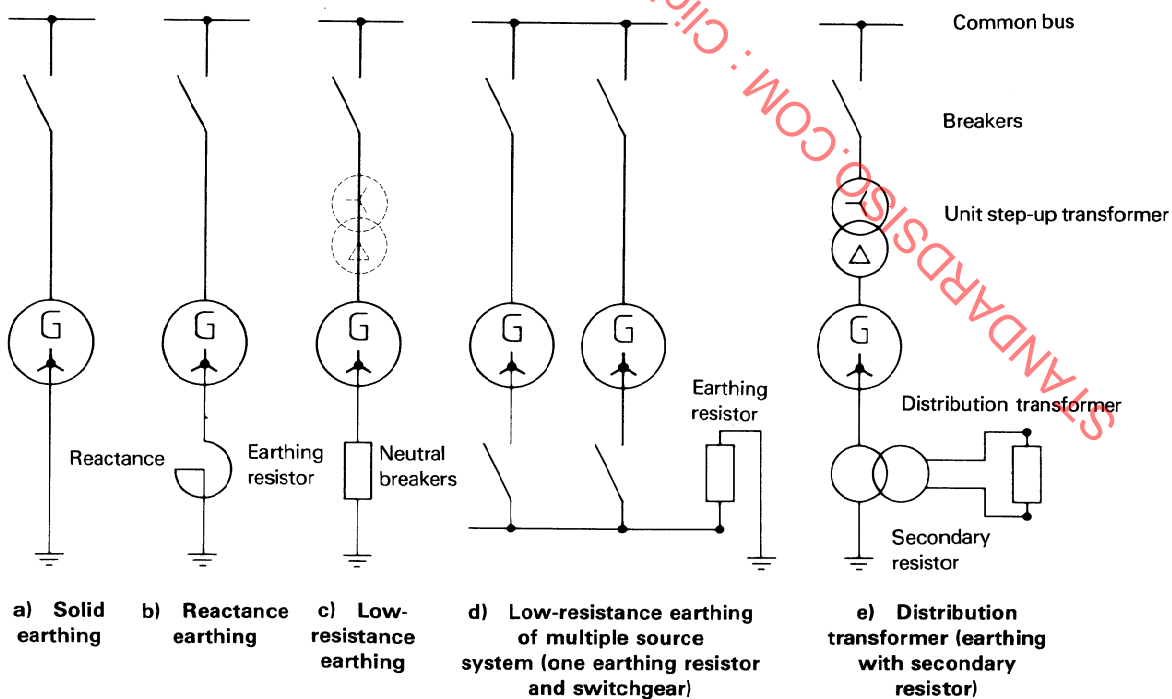
Figure 2 — Generator neutral earthing methods
