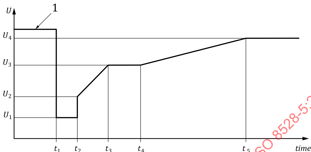
Figure 16 — Example of Voltage against time profile
