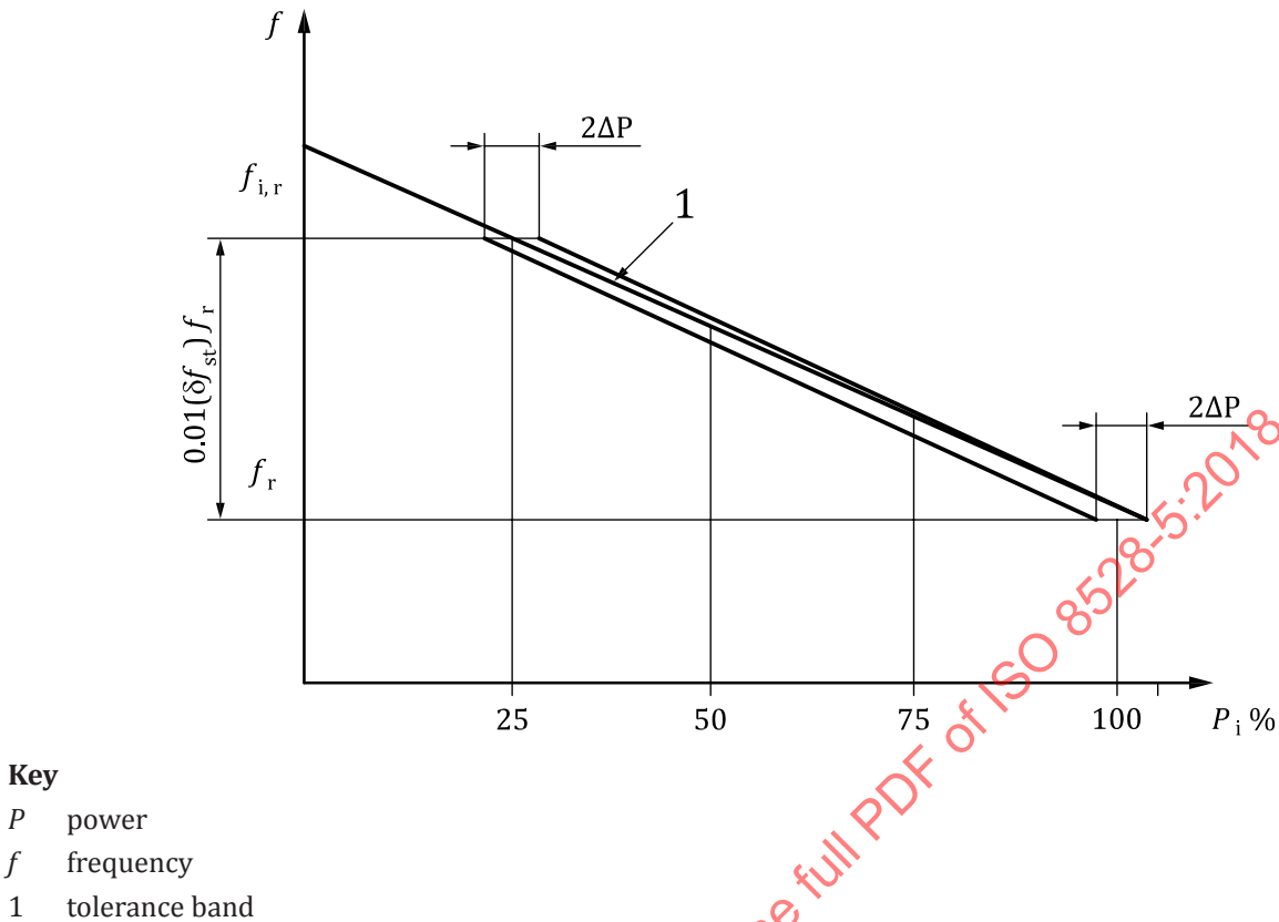
Figure 12 — Example of power sharing in parallel running operation when power limit is 100 % load
