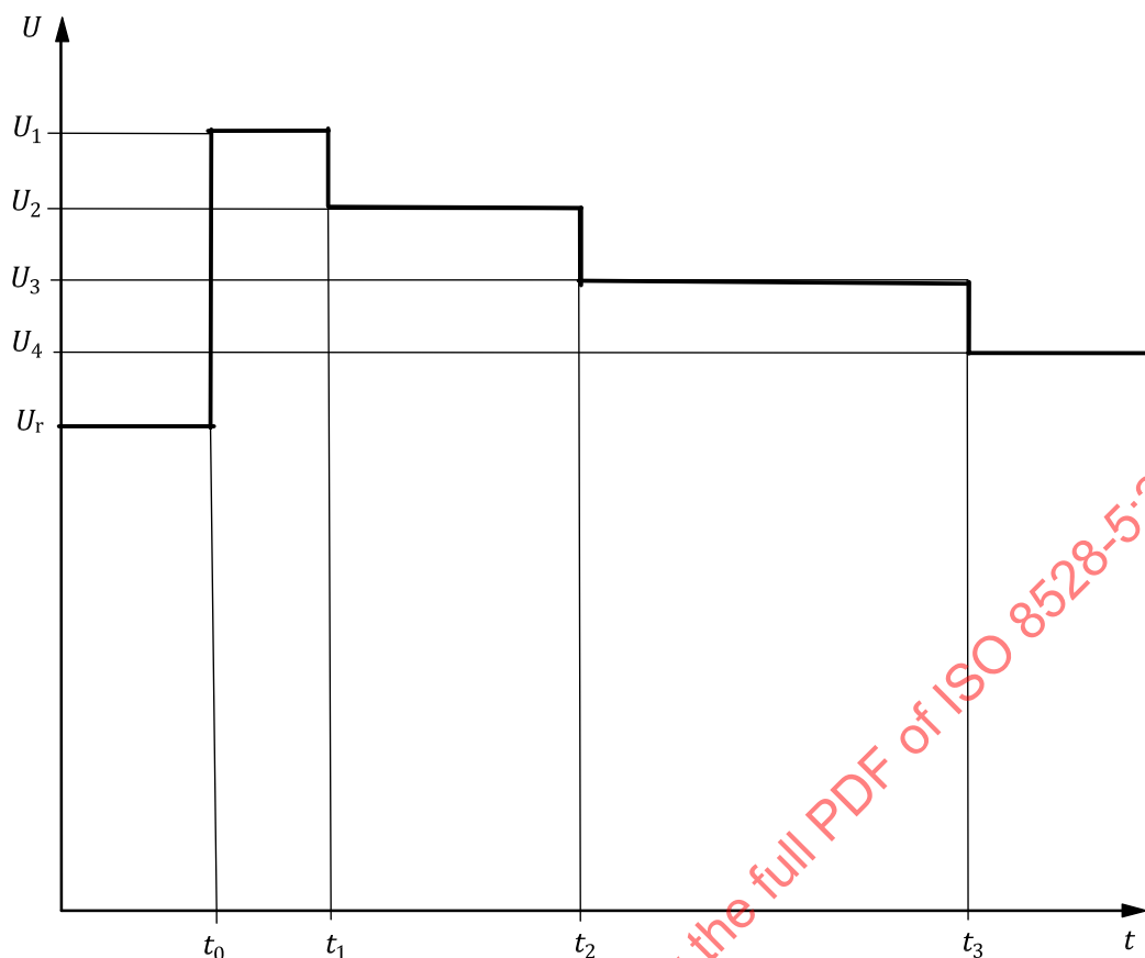
b) Over voltage ride through profile
