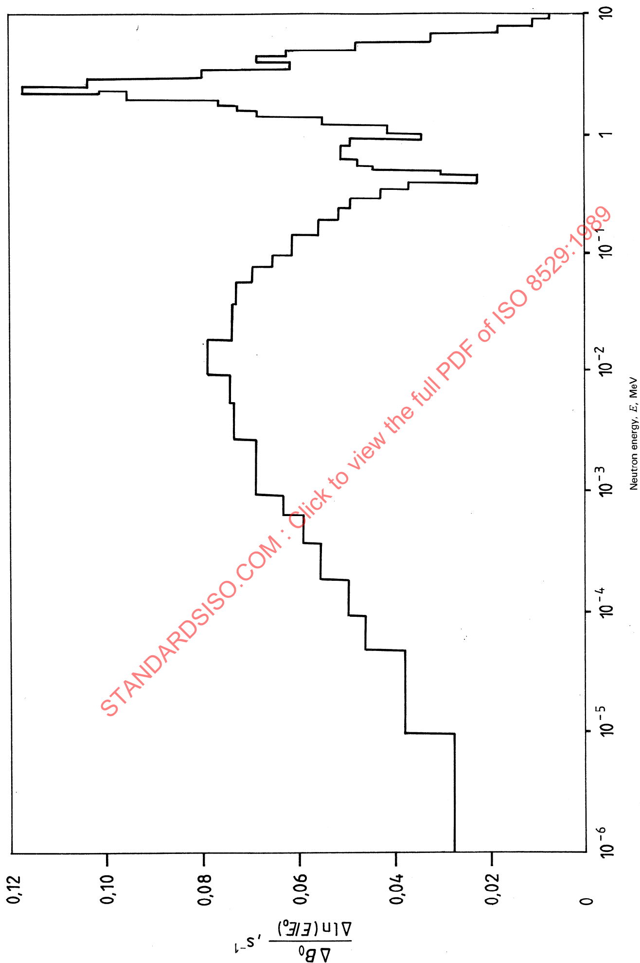
Figure A.3 — Neutron spectrum from a ^{252}\text{Cf} spontaneous fission source in the centre of a \text{D}_2\text{O} sphere with a radius of 150 mm [2]
