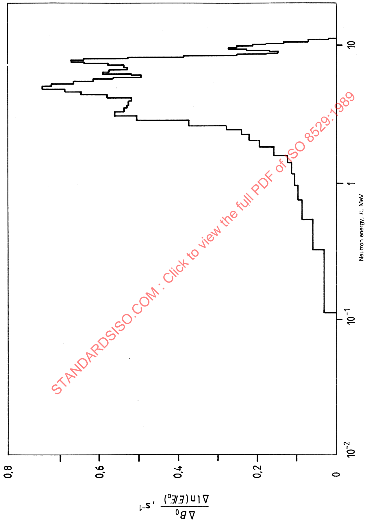
Figure A.2 — Neutron spectrum from a ^{241}\text{Am-Be}(\alpha, n) source [6]
