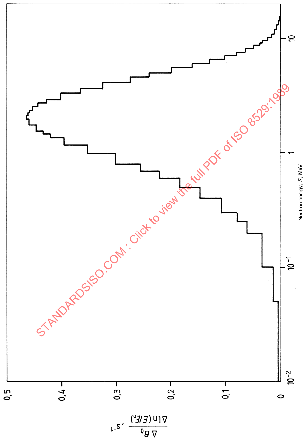
Figure A.1 — Neutron spectrum from a ^{252}\text{Cf} spontaneous fission source (see 4.2.2 and [4])
