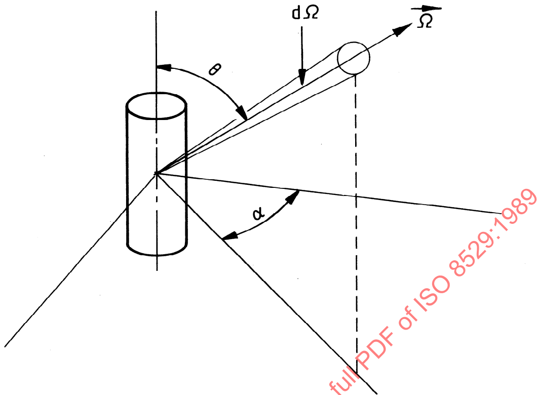
Figure 1 — Coordinate system for the case of an anisotropically emitting source (see 4.3)
