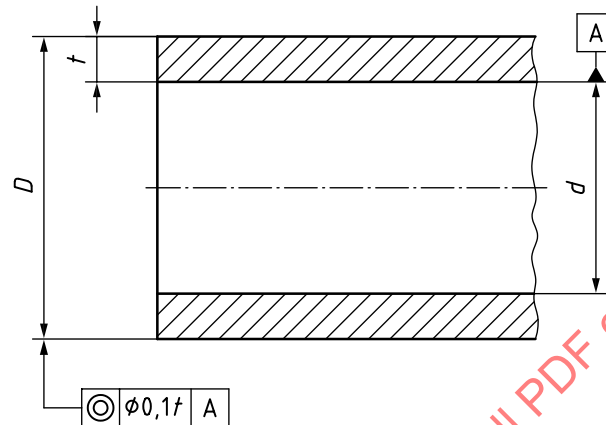
Concentricity of the tube outside diameter
