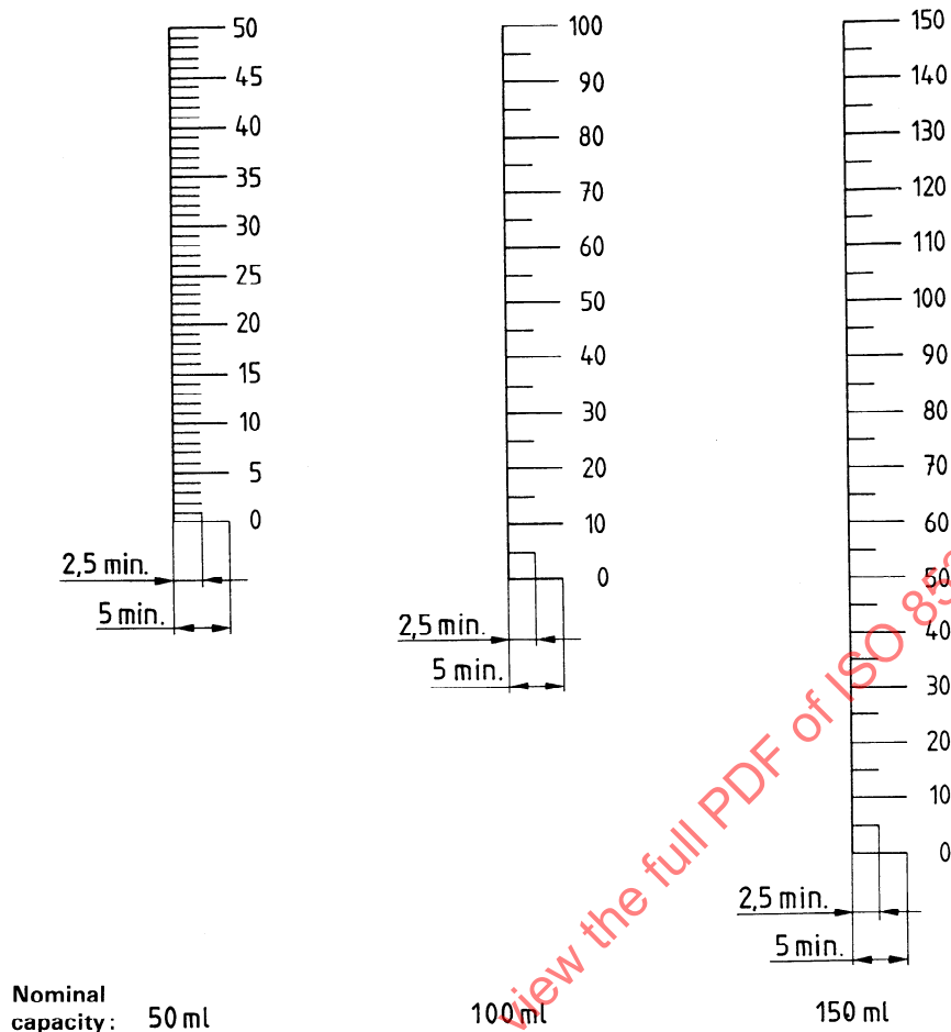
Figure 2 — Typical graduated scales for use in burette sets
