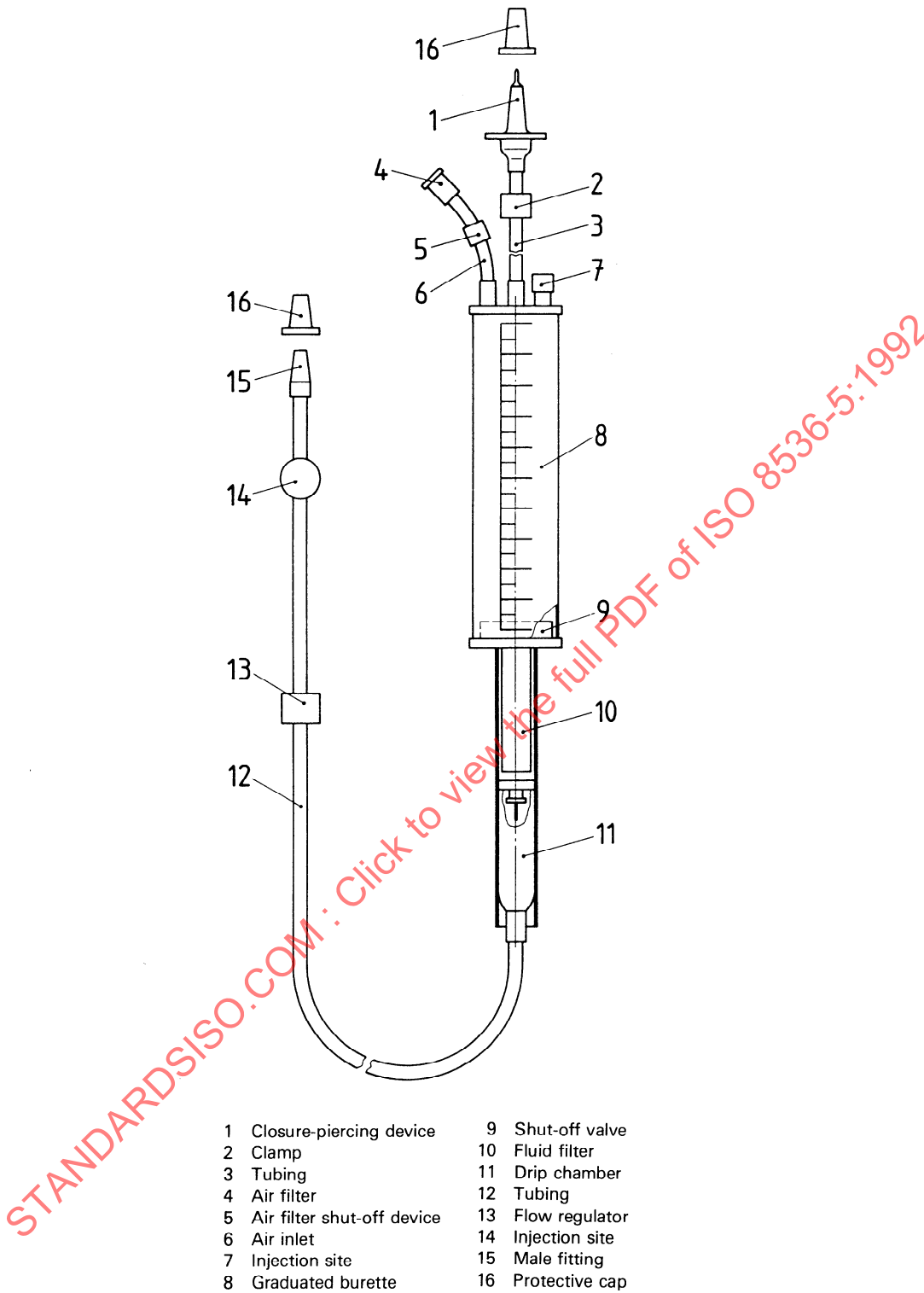
Figure 1 — Example of typical burette set
