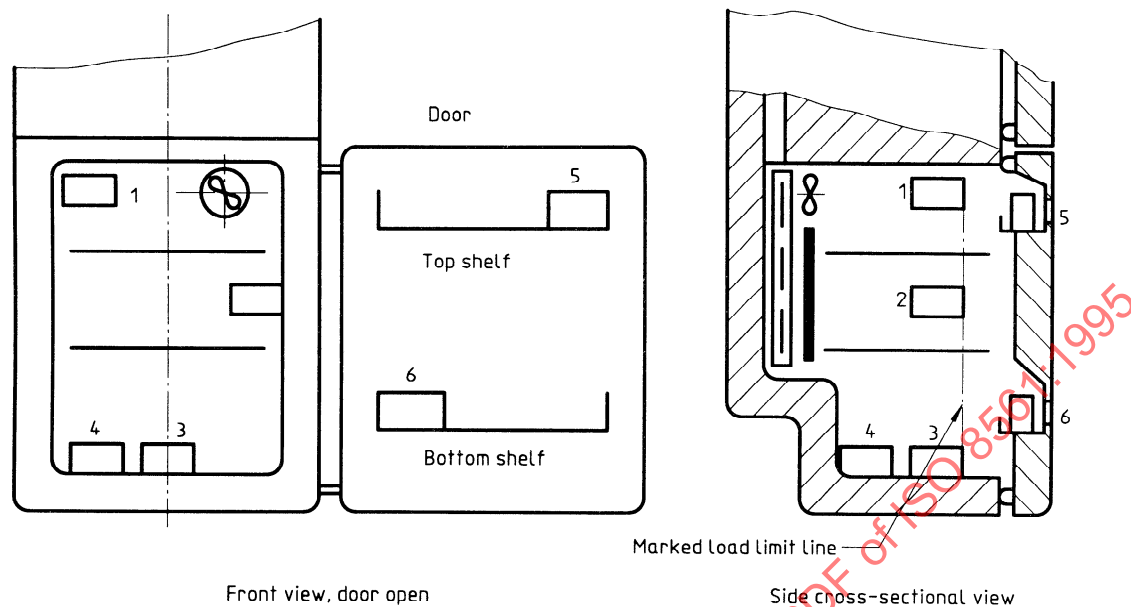
a) Food freezer compartment or frozen food storage compartment - with door storage - with n shelves - with marked load limit line
