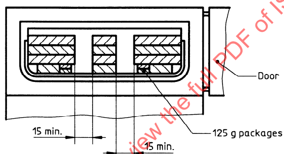
h) Front view, containers with radiused corners
