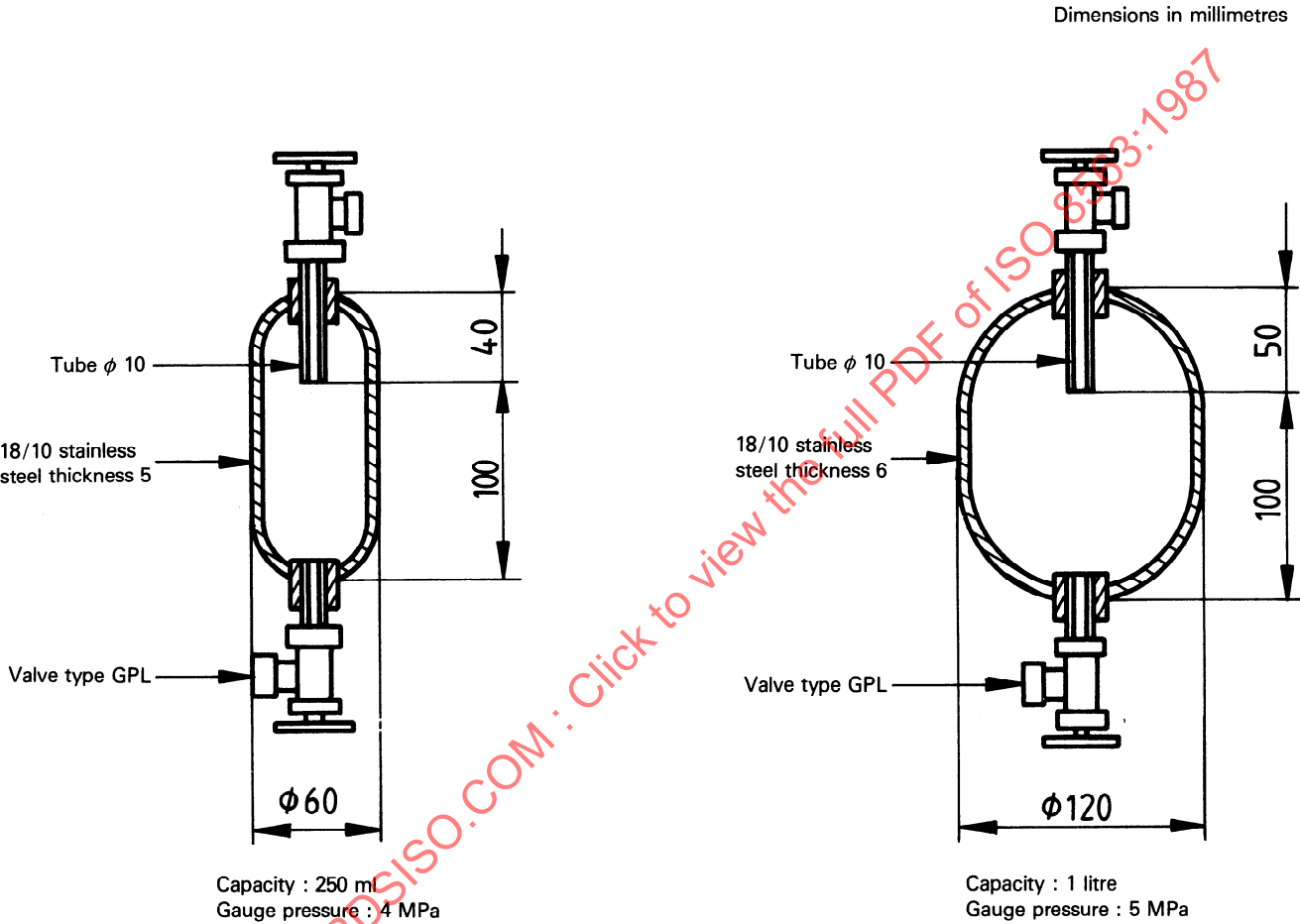
Figure 2 — Examples of sampling cylinders for liquid propylene
