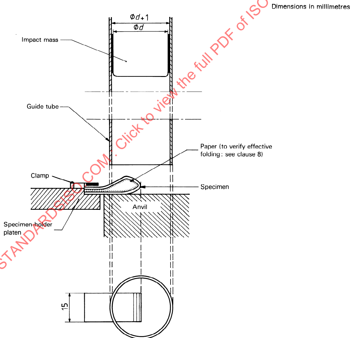
Figure 1 — Typical impact device for determination of cold-crack temperature
