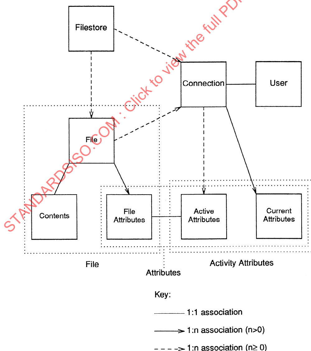
Figure 7 — Virtual filestore schema
