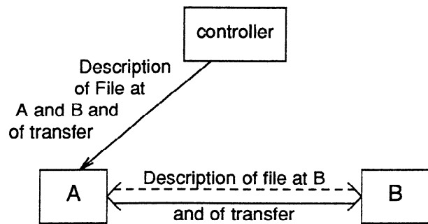
Figure 2b - Actual flows of information in FTAM
