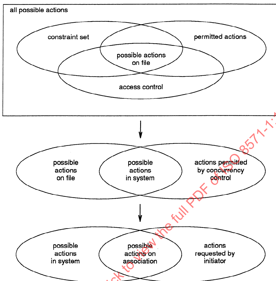
Figure 5 — Restrictions on the possible actions
