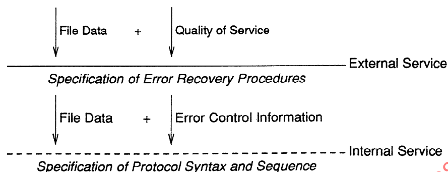
Figure 4 — Structuring a file protocol entity
