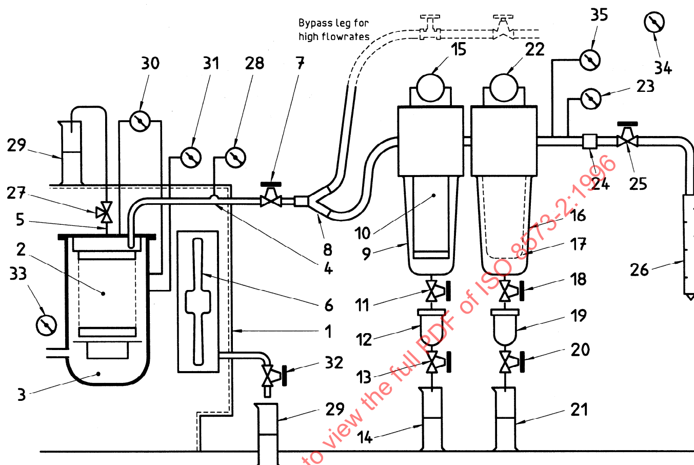
Figure 2 — Apparatus for Test Method A
