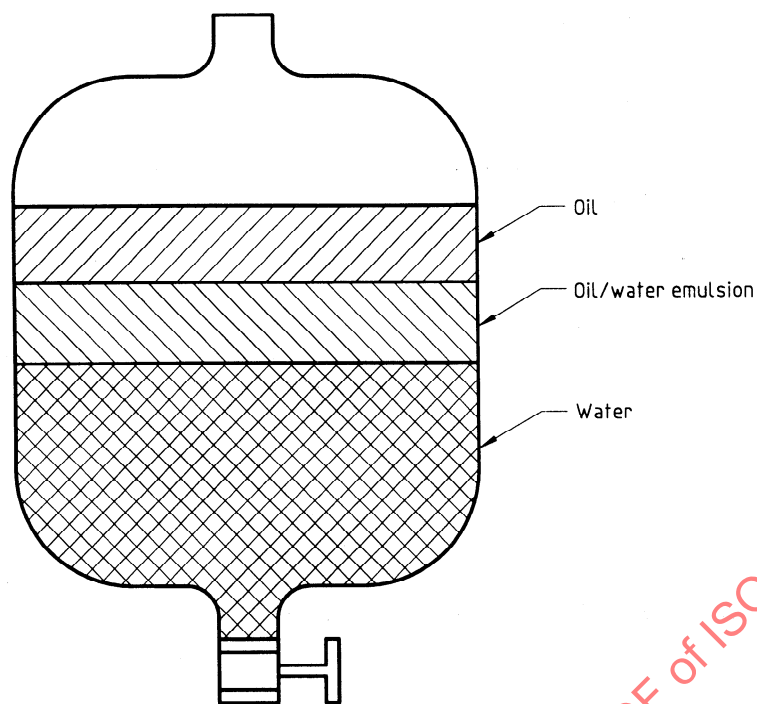
Figure 8 — Oil/water separator
