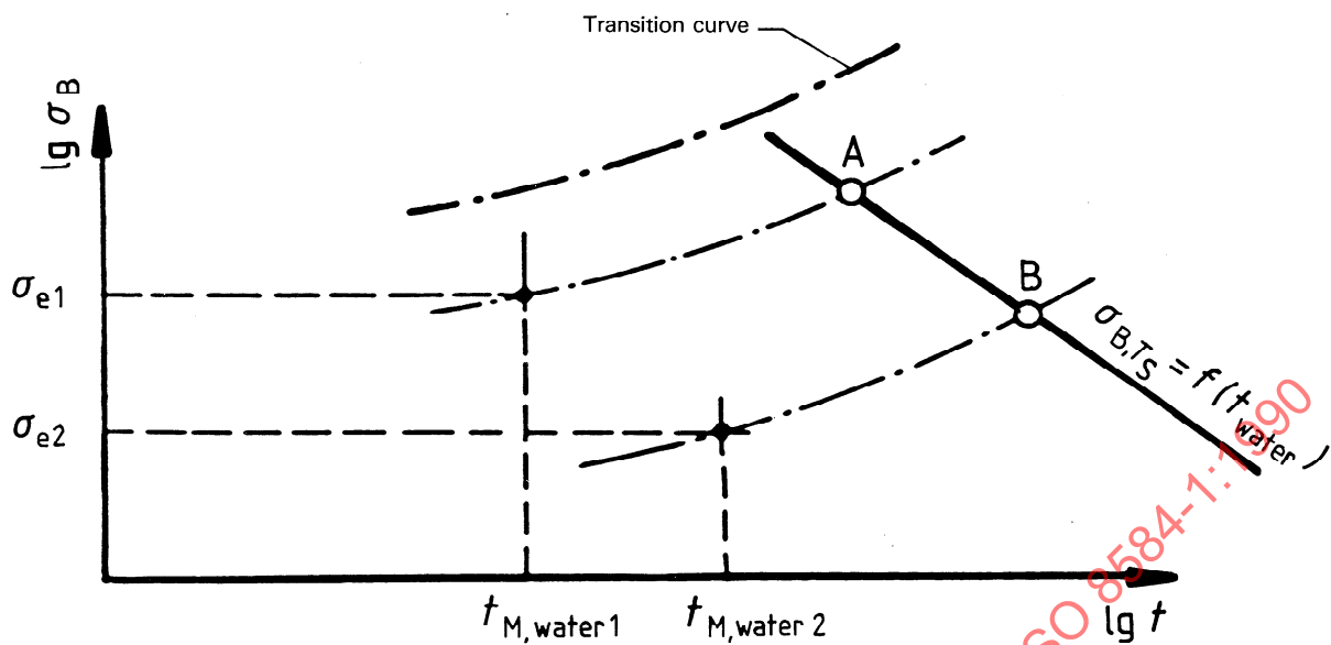
Figure 2 — Graphical representation of the reference points derived from the measurement points
