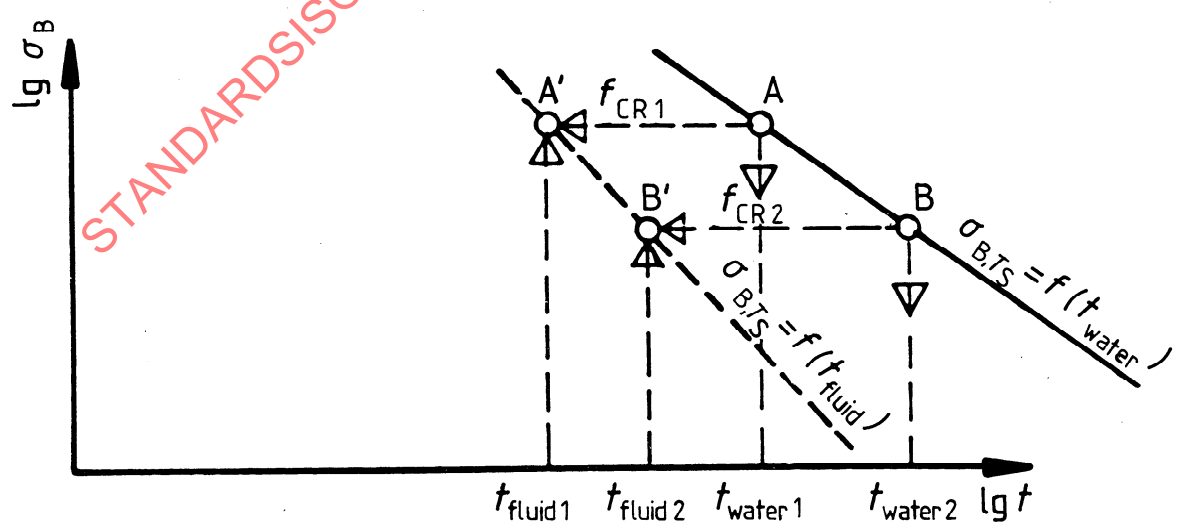
Figure 3 — Graphical representation of the basic stress line for a fluid
