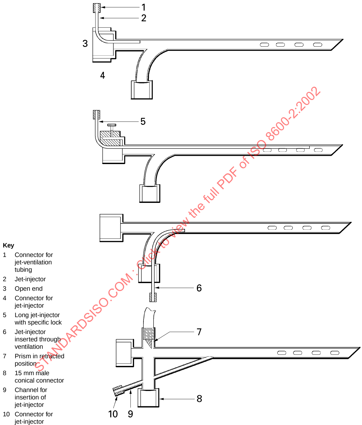
Figure 2 — Examples of rigid jet-ventilation bronchoscopes
