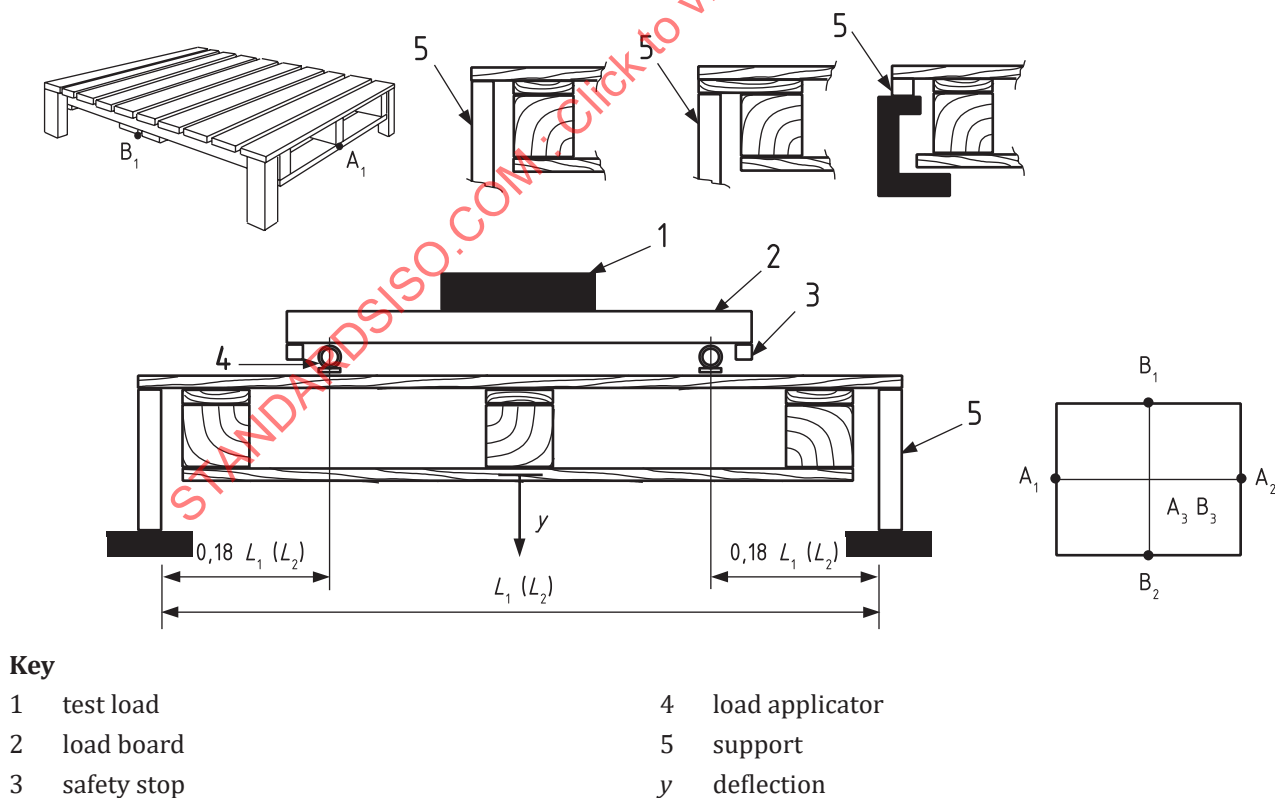
Figure 6 — Wing pallet bending test
