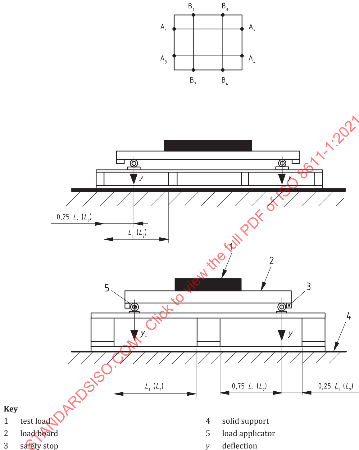
Figure 5 — Bottom deck strength and stiffness test
