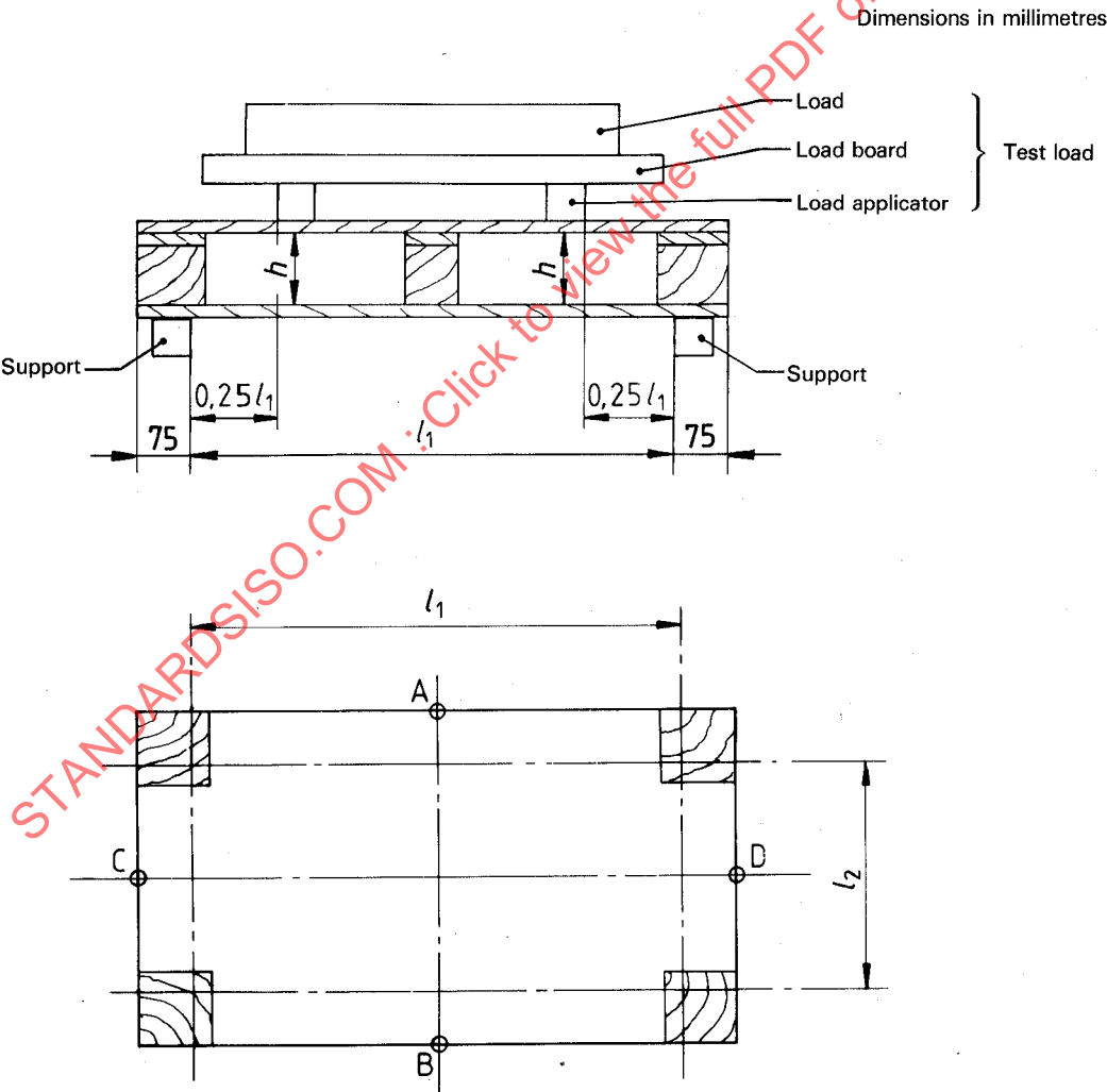
Figure 2 — Bending test using square supports and load applicators (see also figure 3)
