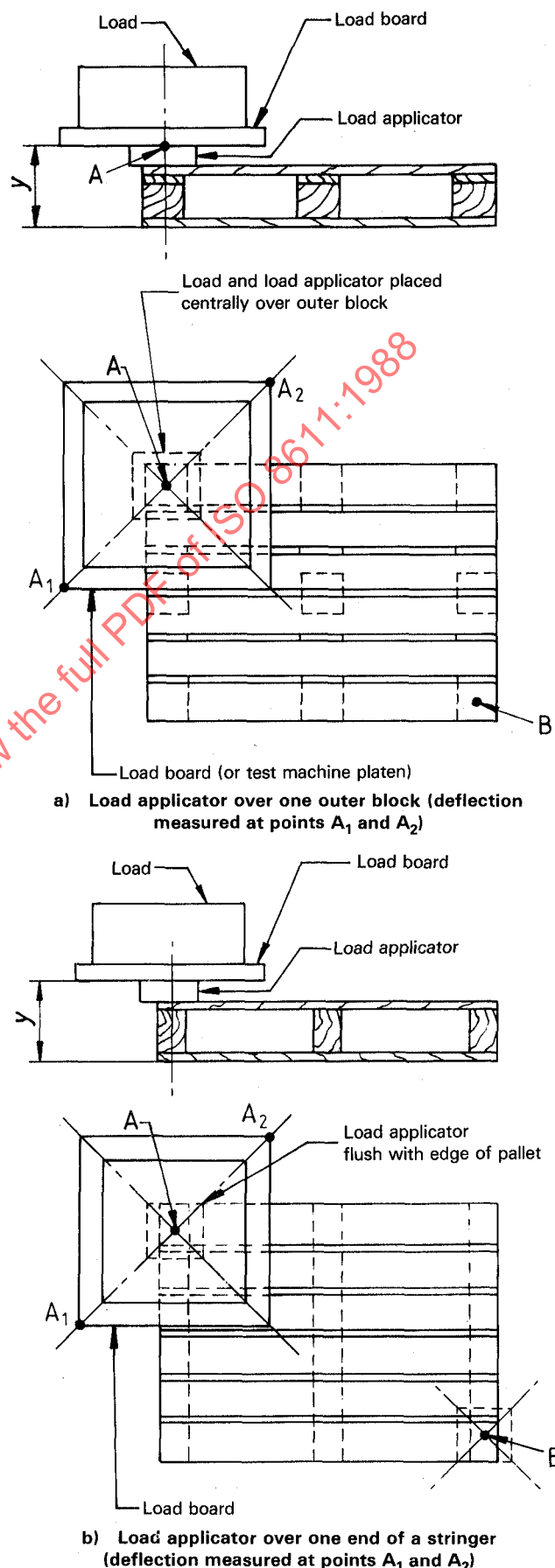
Figure 1 — Stacking test
