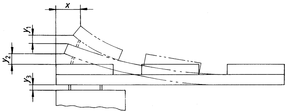
Figure 8 — Top deck edge impact test — Points of measurement
