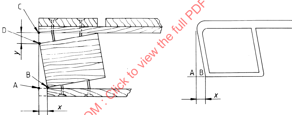
Figure 7 — Shear test — Points of measurement
