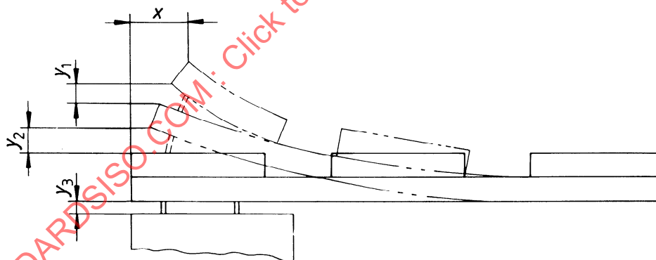
Figure 9 — Top deck edge impact test — Points of measurement
