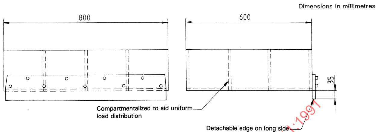
Figure 6 — Load box for inclined-plane tests
