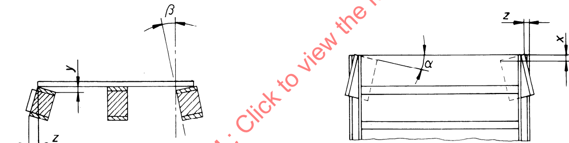
Figure 12 — Displacements x , y and z and angles \alpha and \beta
