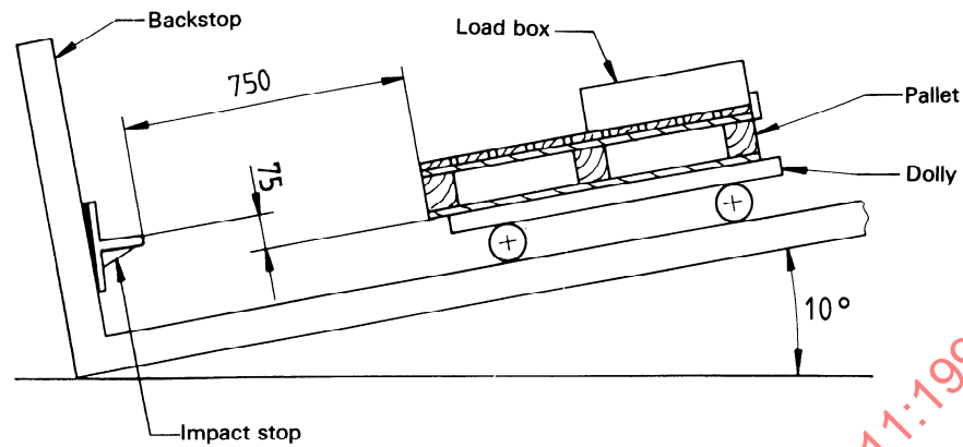
a) Position before release
