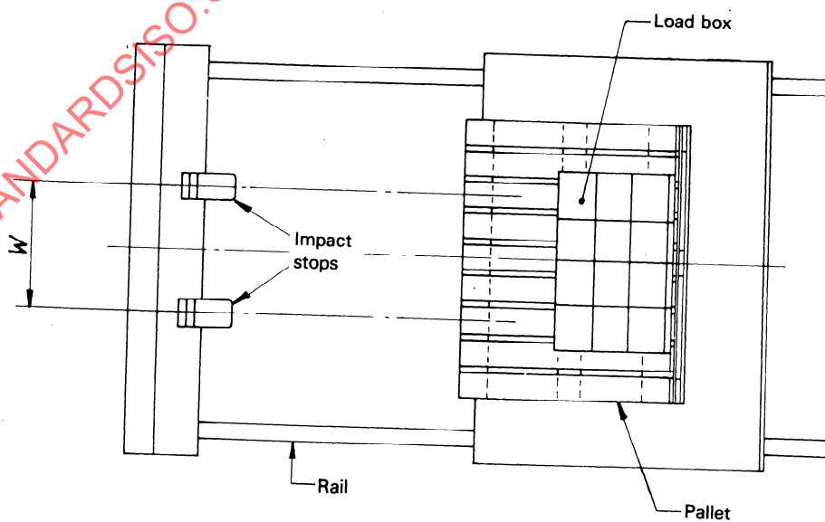
c) Plan view of position before release
