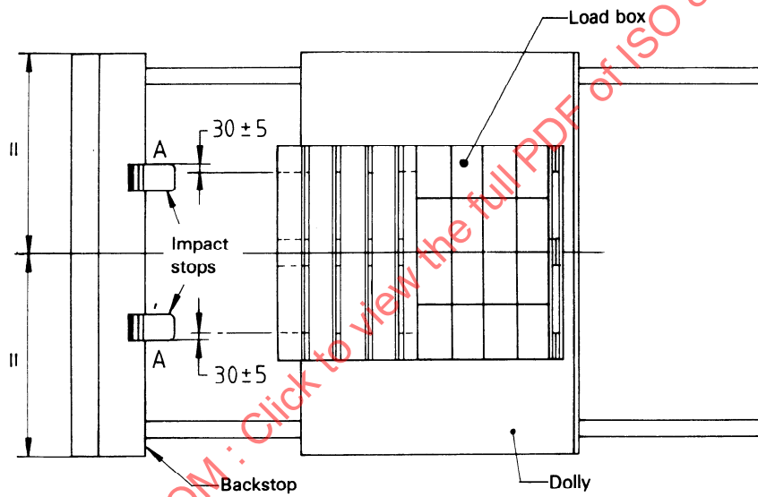
b) Plan view showing position of blocks
