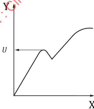
Figure A.1 — Force versus deformation plot indicating total pallet failure
