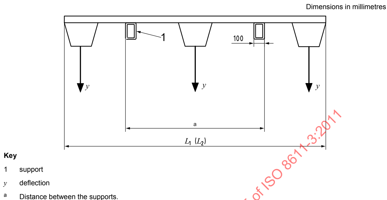
Figure 2 — Test 2b — Forklifting test
