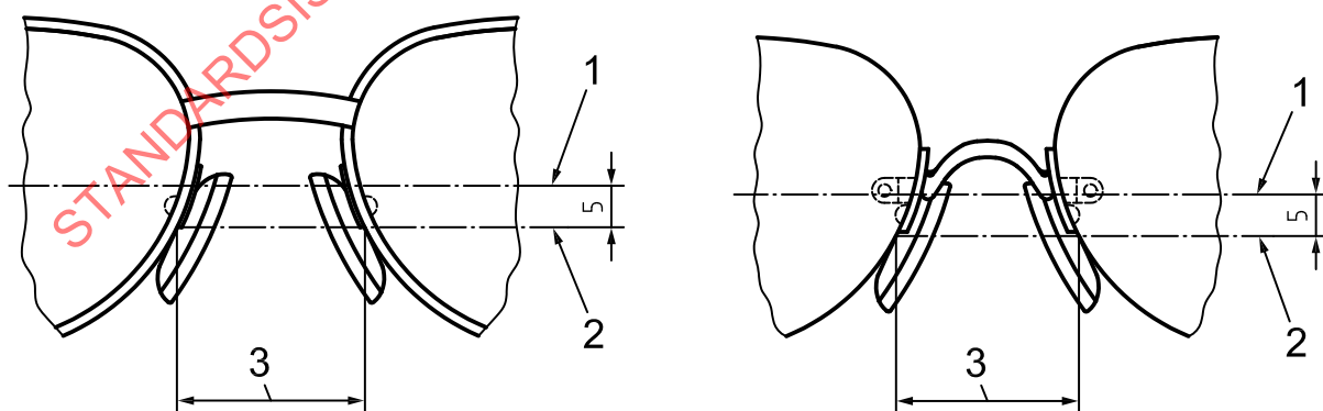
a) Spectacle frames with metal pad bridges
