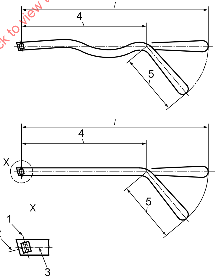
Figure 2 — Measurements related to spectacle frames — Spectacle sides
