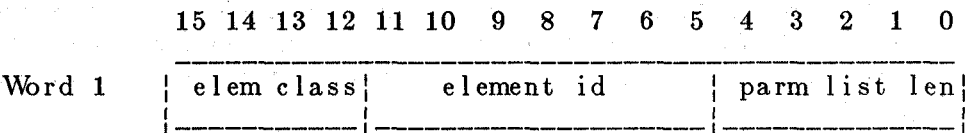
Figure 1 — Format of a short-form Command Header.
