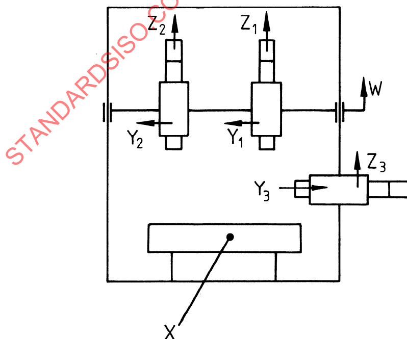
Figure 3 — Type 2: Machine with three milling heads
