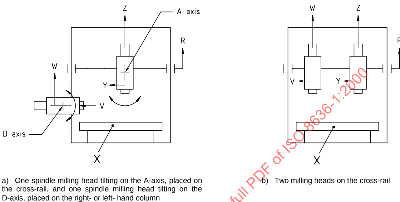
Figure 2 — Type 1: Machines with two milling heads
